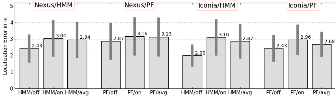
Figure 6.7 The Device Adaptation shows no effect on the error rates of the Nexus.
